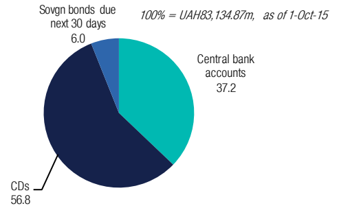
Chart 6. Breakdown of liquidity pool (%) as of 1 Oct 2015
